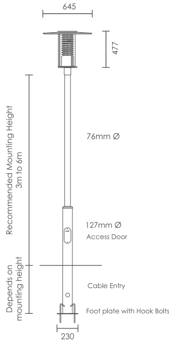
Voyager 3 Post Top LED version on Stepped Modern Pole Buried
