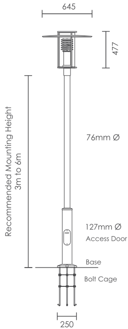
Voyager 3 Post Top on Stepped Modern Pole Plinth
