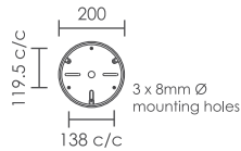
Wall Mounting Plate Detail
