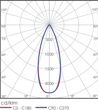
LED 4W 35° Beam
