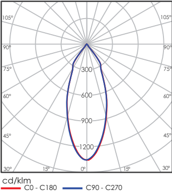
LED 13W 40° Beam
