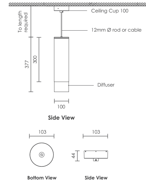
Ceiling Cup 100 Ceiling cup 100 with suspension tube and cable Ceiling cup 100 with suspension cable only
