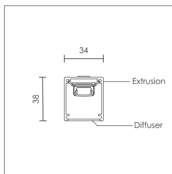
Section View Profile
