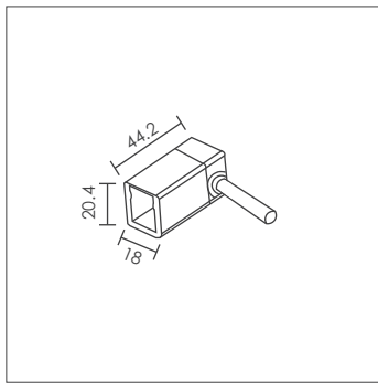
QUICK CONNECTOR WITH WIRE IN THE MIDDLE
