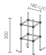
Grand Classic Post Bolt Cage M12 Threaded Rod
