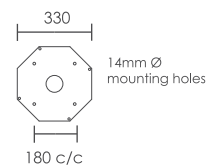
Grand Classic Post Base Plate Detail
