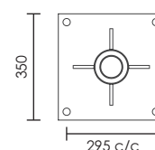
BASE PLATE DETAIL 350x350x16
