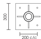
BASE PLATE DETAIL 300x300x10
