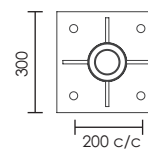
BASE PLATE DETAIL 300x300x10
