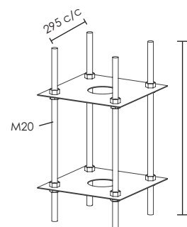
BOLT CAGE M20-750 M20 Threaded Rod
