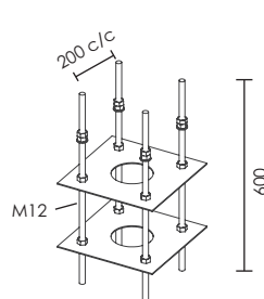
BOLT CAGE M12-600 M12 Threaded Rod
