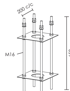
BOLT CAGE M16-650 M16 Threaded Rod
