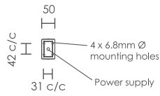
Mounting Plate Detail
