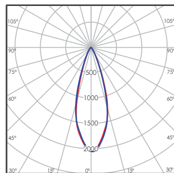
LED 10W 36°
