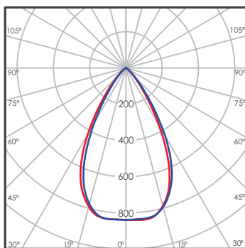
LED 10W 60°
