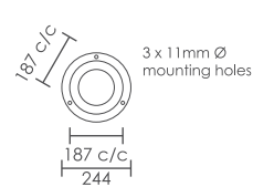
Century Post Base Detail
