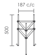
Century Post Bolt Cage M10 Threaded Rod
