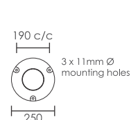
Stepped Modern Base Detail
